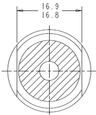
VIEW AT A-A
